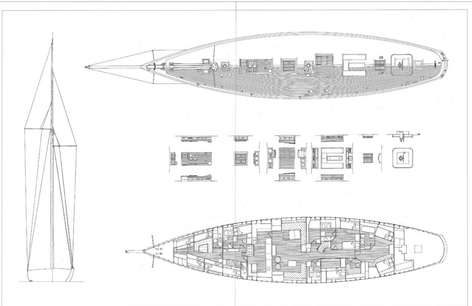
Detailed drawing of the accommodations, deck, and rigging of Morrite - 1995 version, by François Chevalier (©2010 François Chevalier)
